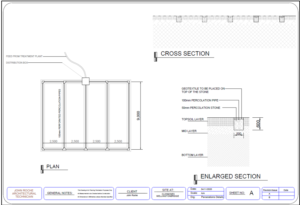
Figure 17. Details of the proposed percolation area. (Source: 2020 Site Suitability Assessment, John Roche Architectural Services)
